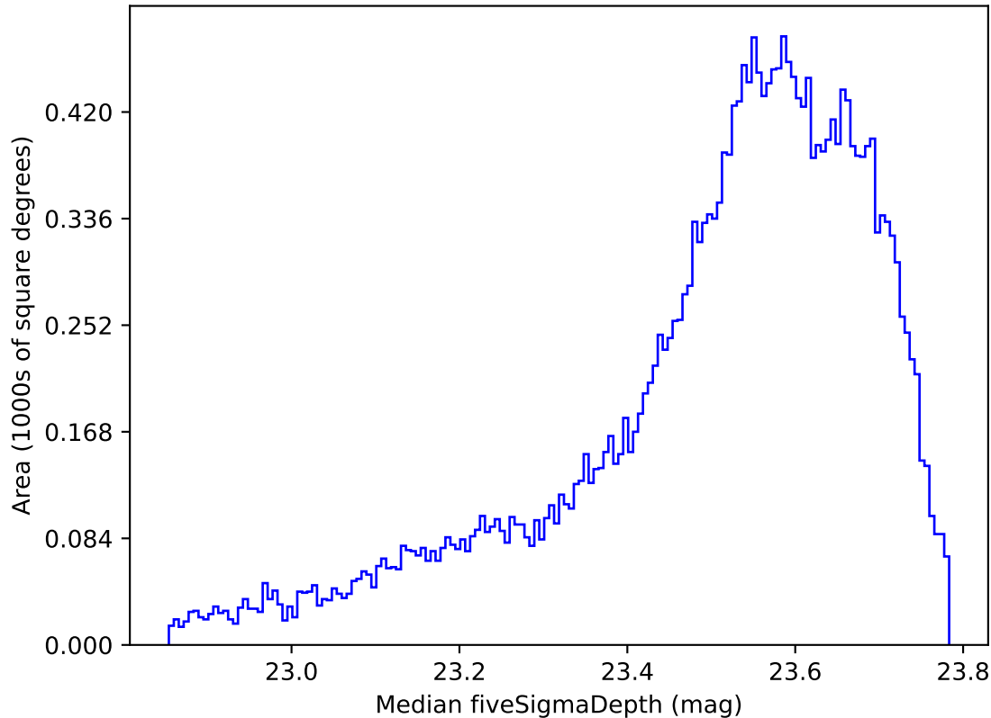
ddf_acor_sf15_lsf40_lsr20_v3.4_10yrs All sky i band: Median fiveSigmaDepth
