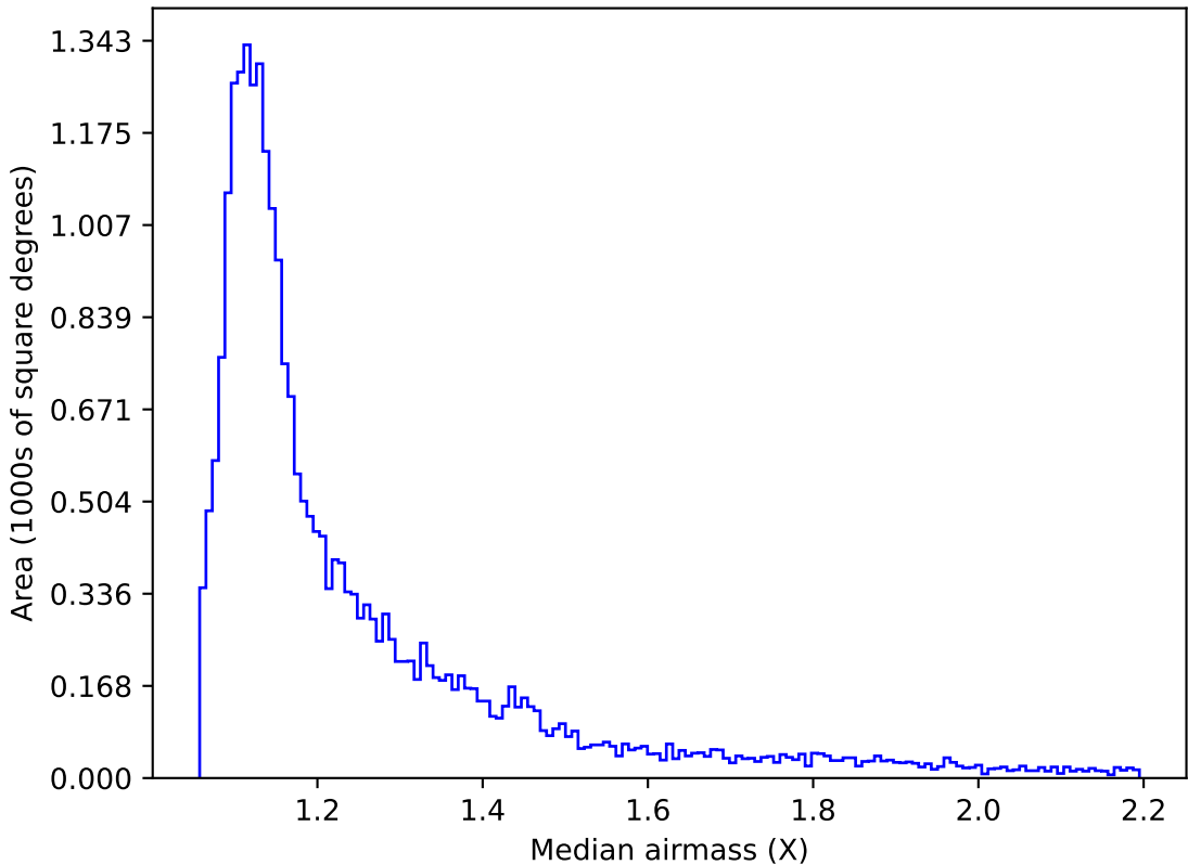
ddf_acor_sf15_lsf40_lsr20_v3.4_10yrs Yr 1 z band: Median airmass
