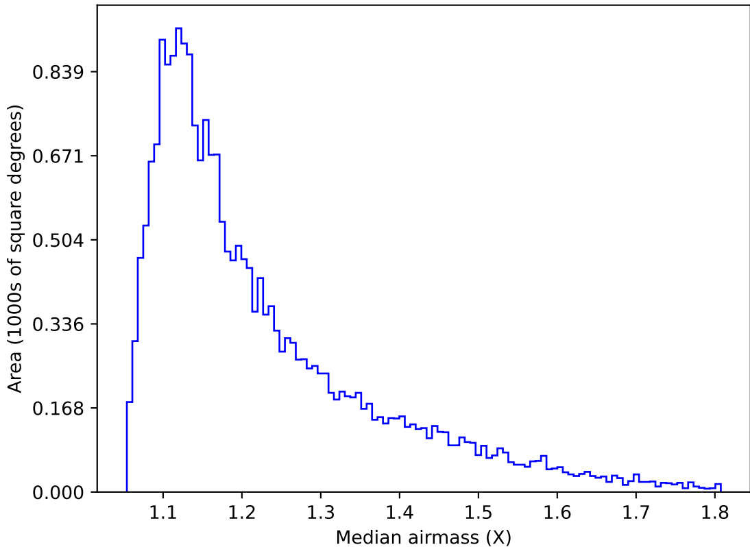
ddf_acor_sf15_lsf40_lsr20_v3.4_10yrs Yr 1 u band: Median airmass
