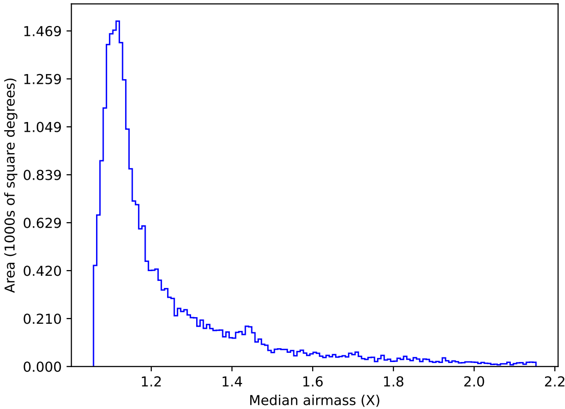
ddf_acor_sf15_lsf40_lsr20_v3.4_10yrs Yr 1 i band: Median airmass
