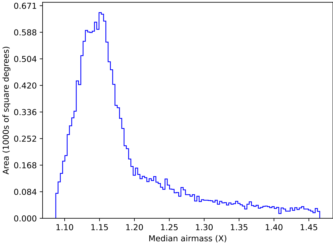
ddf_acor_sf15_lsf40_lsr20_v3.4_10yrs WFD z band: Median airmass
