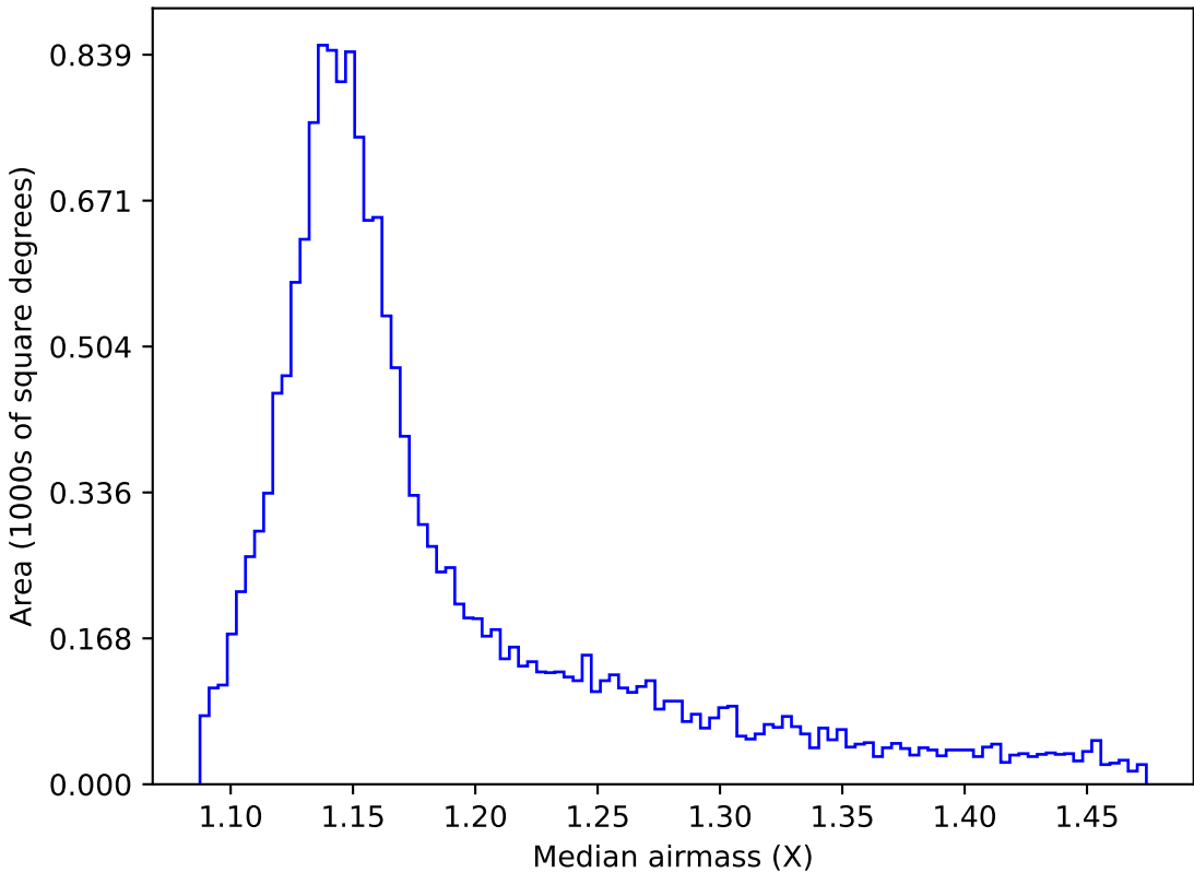
ddf_acor_sf15_lsf40_lsr20_v3.4_10yrs WFD y band: Median airmass
