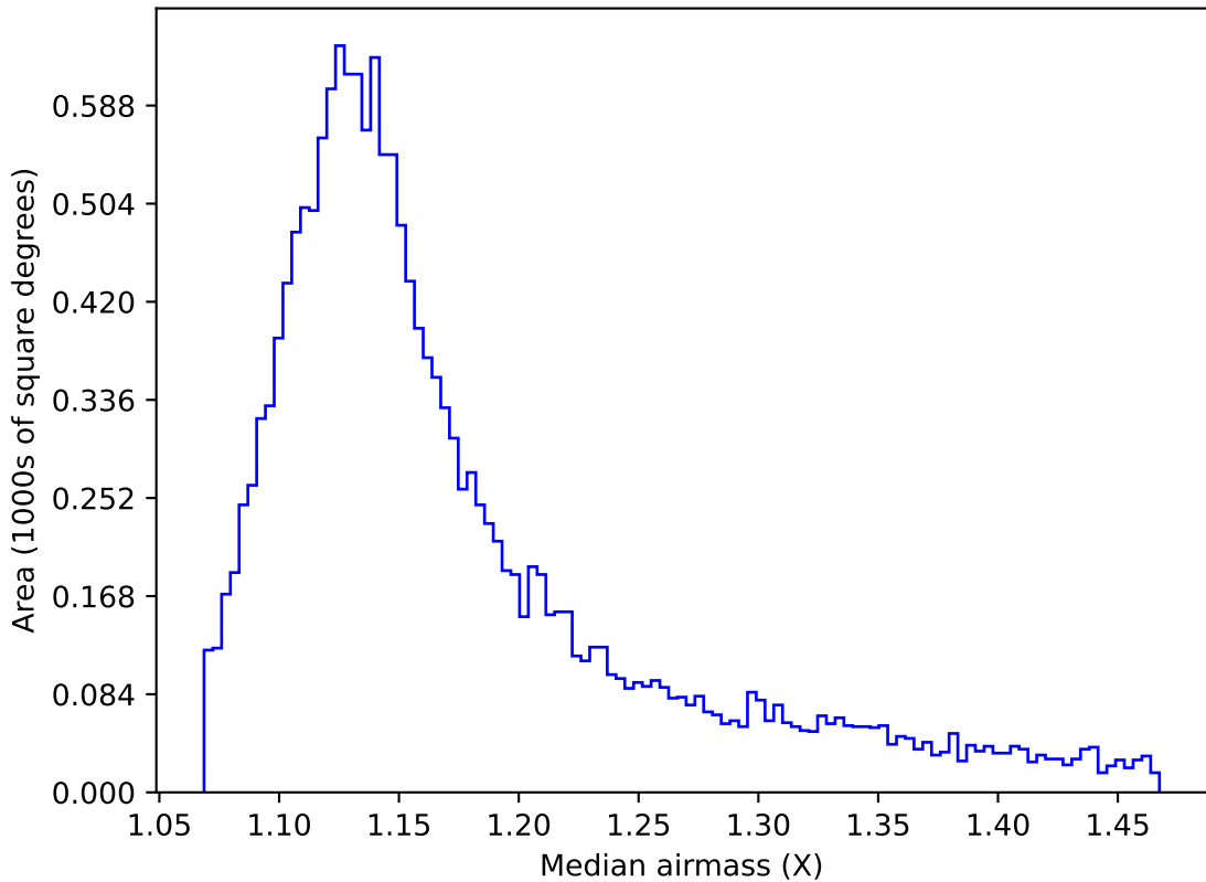
ddf_acor_sf15_lsf40_lsr20_v3.4_10yrs WFD u band: Median airmass
