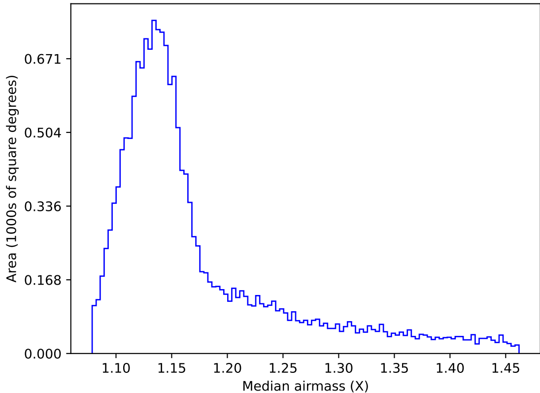
ddf_acor_sf15_lsf40_lsr20_v3.4_10yrs WFD i band: Median airmass
