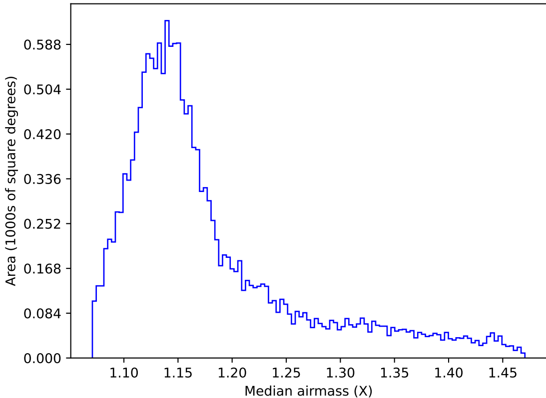
ddf_acor_sf15_lsf40_lsr20_v3.4_10yrs WFD g band: Median airmass
