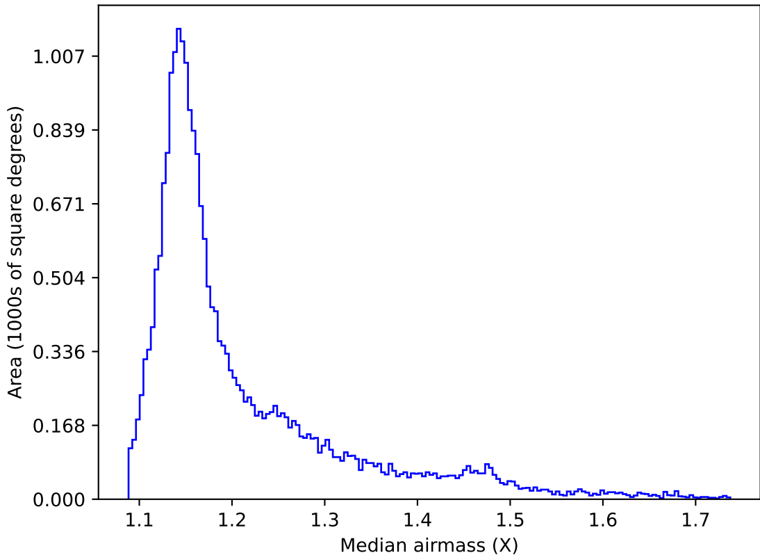
ddf_acor_sf15_lsf40_lsr20_v3.4_10yrs All sky y band: Median airmass
