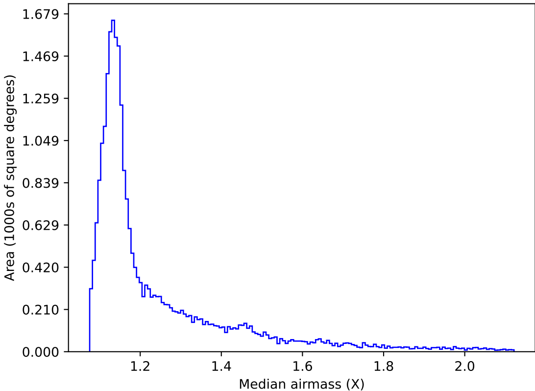
ddf_acor_sf15_lsf40_lsr20_v3.4_10yrs All sky r band: Median airmass
