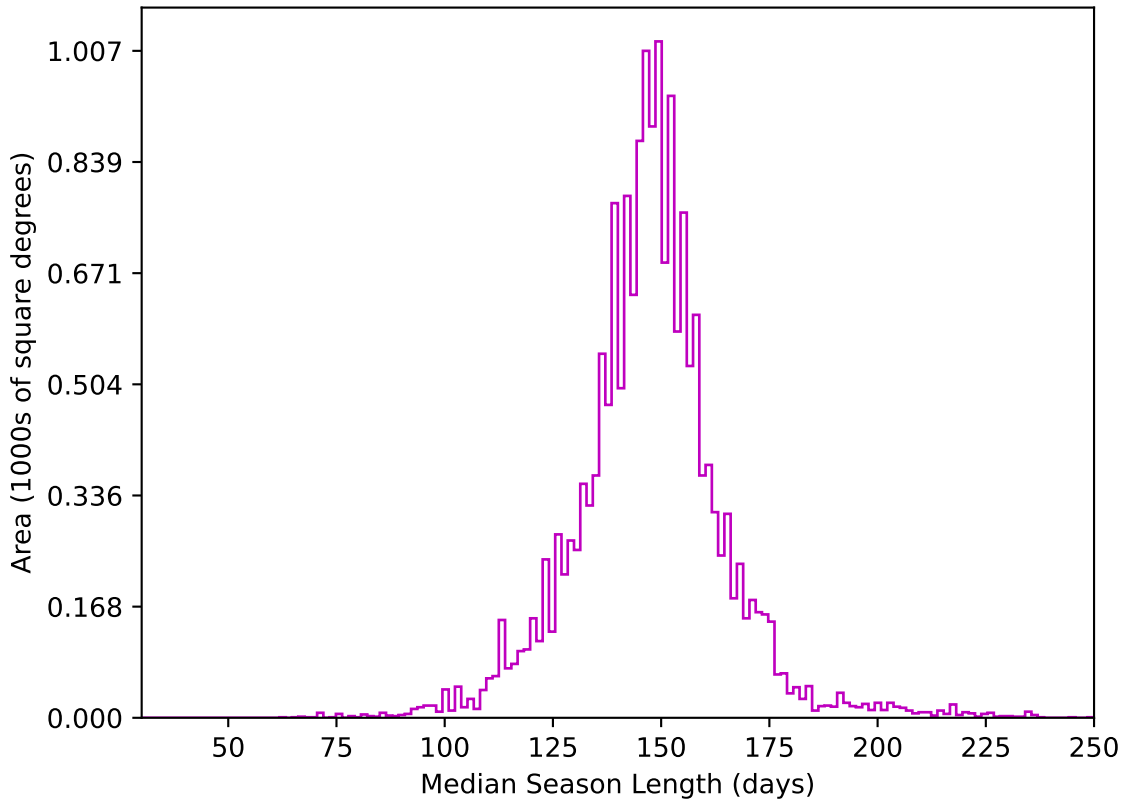
ddf_acor_sf15_lsf40_lsr20_v3.4_10yrs WFD z band: Median Season Length
