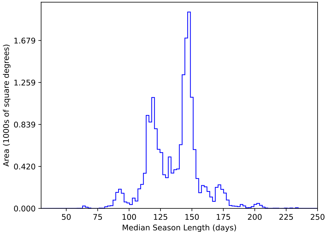
ddf_acor_sf15_lsf40_lsr20_v3.4_10yrs WFD y band: Median Season Length
