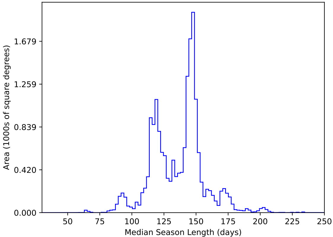
ddf_acor_sf15_lsf40_lsr20_v3.4_10yrs WFD y band: Median Season Length
