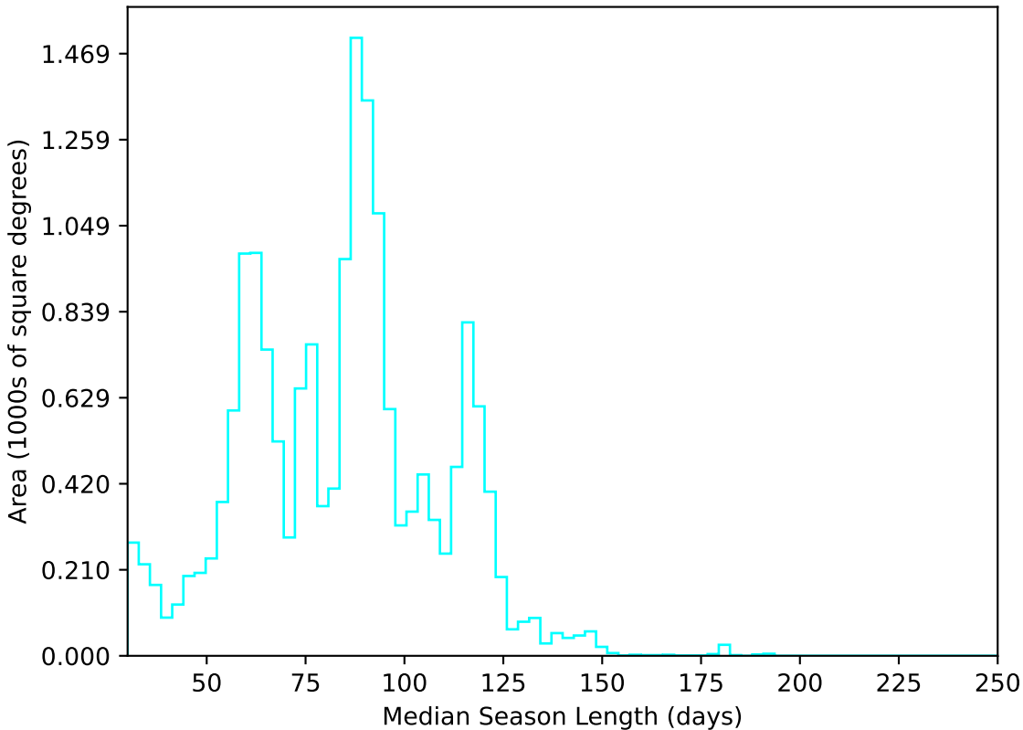
ddf_acor_sf15_lsf40_lsr20_v3.4_10yrs WFD u band: Median Season Length
