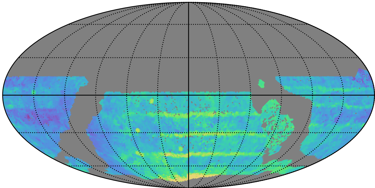
ddf_acor_sf15_lsf40_lsr20_v3.4_10yrs WFD all bands: Median Season Length
