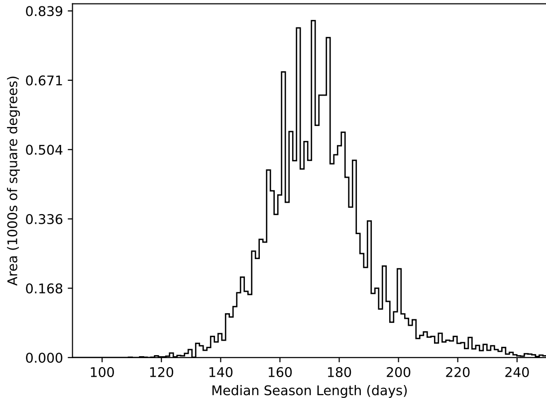
ddf_acor_sf15_lsf40_lsr20_v3.4_10yrs WFD all bands: Median Season Length
