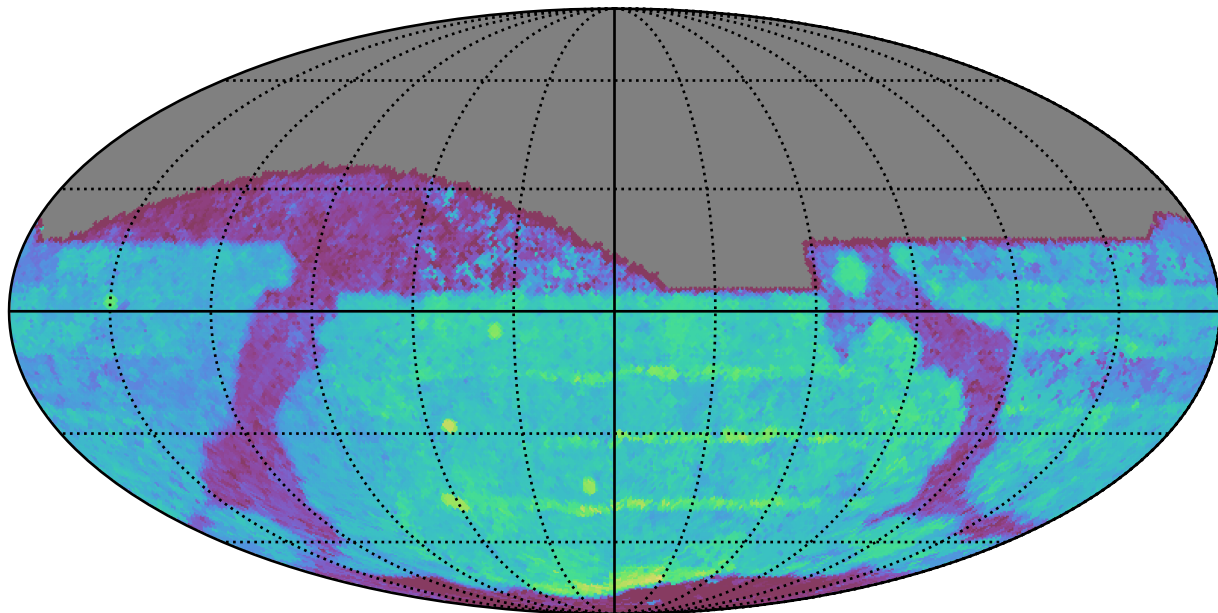
ddf_acor_sf15_lsf40_lsr20_v3.4_10yrs All sky z band: Median Season Length
