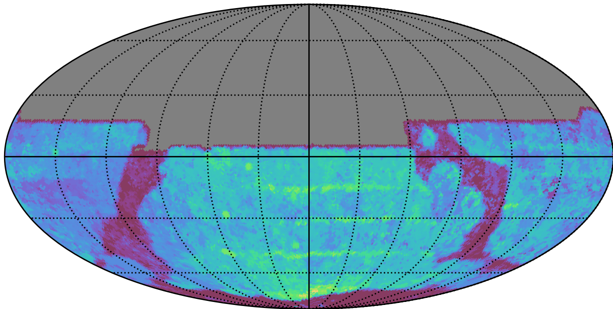
ddf_acor_sf15_lsf40_lsr20_v3.4_10yrs All sky y band: Median Season Length
