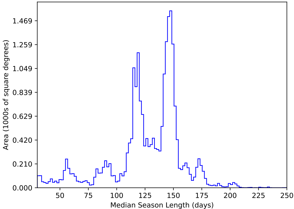
ddf_acor_sf15_lsf40_lsr20_v3.4_10yrs All sky y band: Median Season Length
