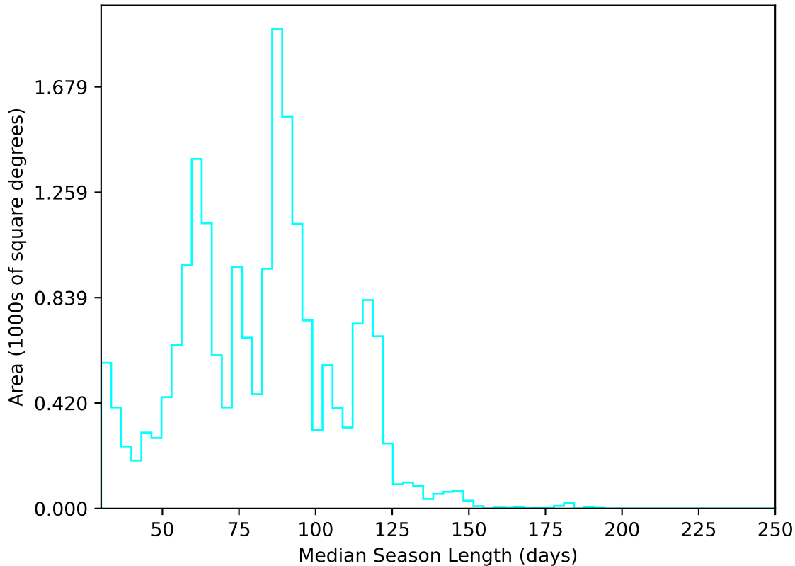
ddf_acor_sf15_lsf40_lsr20_v3.4_10yrs All sky u band: Median Season Length
