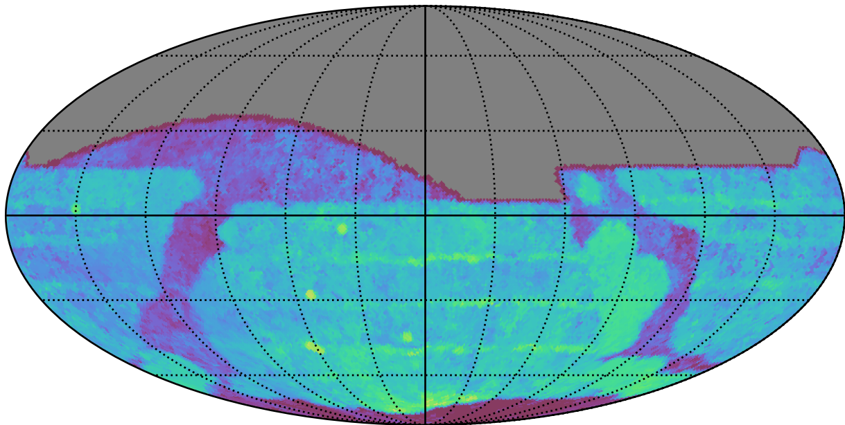
ddf_acor_sf15_lsf40_lsr20_v3.4_10yrs All sky r band: Median Season Length
