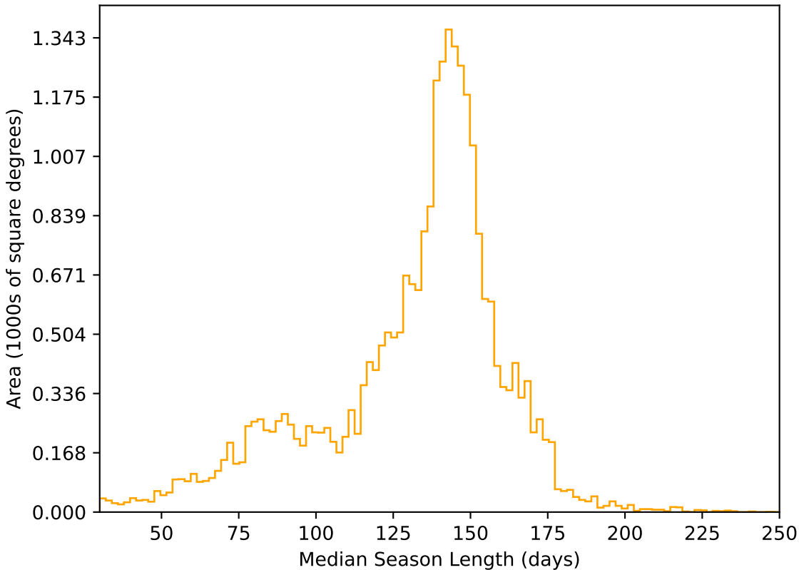
ddf_acor_sf15_lsf40_lsr20_v3.4_10yrs All sky r band: Median Season Length
