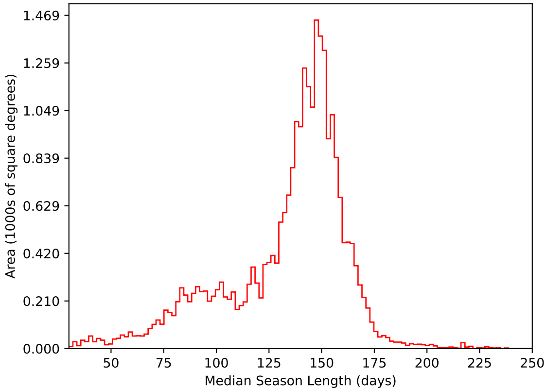
ddf_acor_sf15_lsf40_lsr20_v3.4_10yrs All sky i band: Median Season Length
