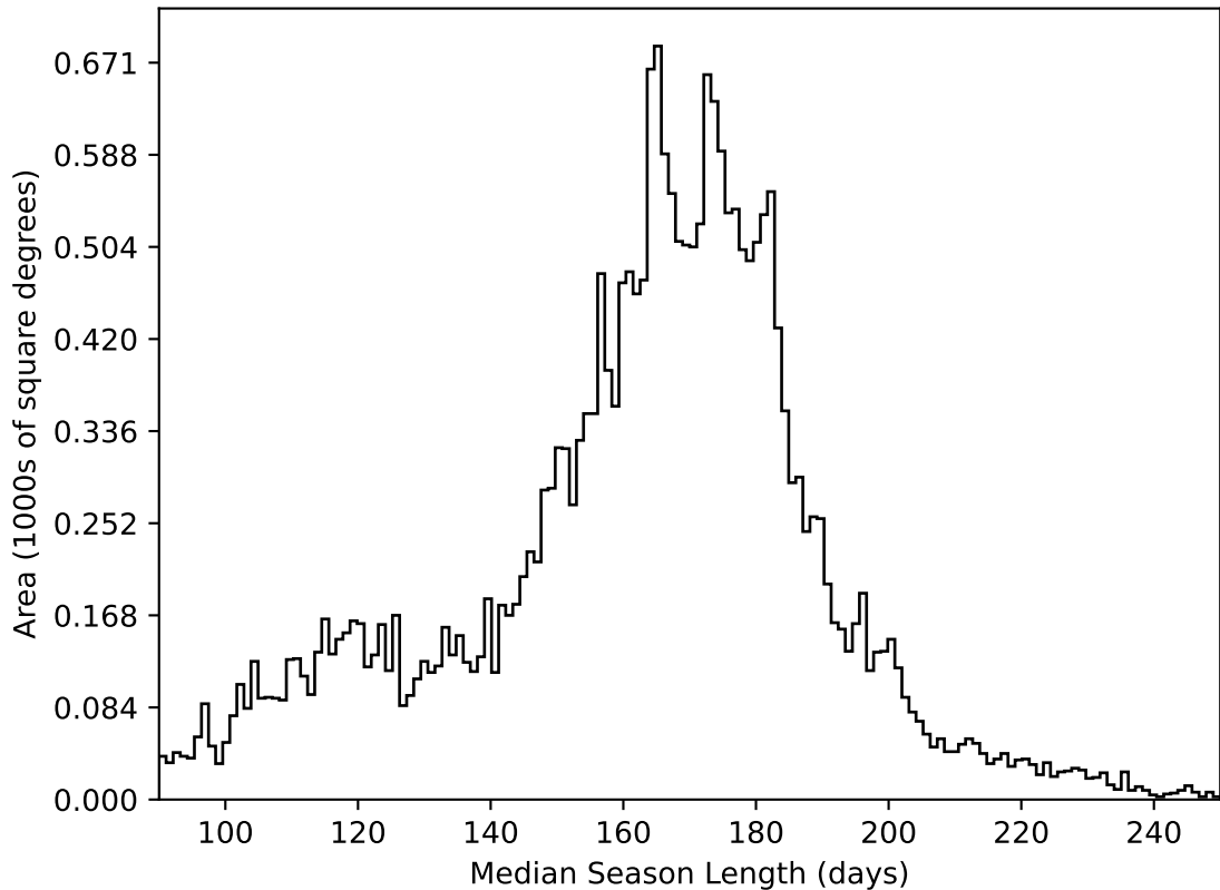
ddf_acor_sf15_lsf40_lsr20_v3.4_10yrs All sky all bands: Median Season Length
