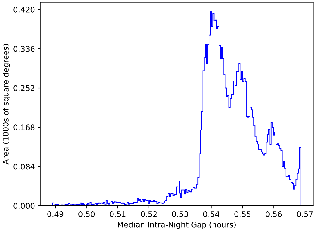
ddf_acor_sf15_ls40_lsr20_v3.4_10yrs WFD: Median Intra-Night Gap
