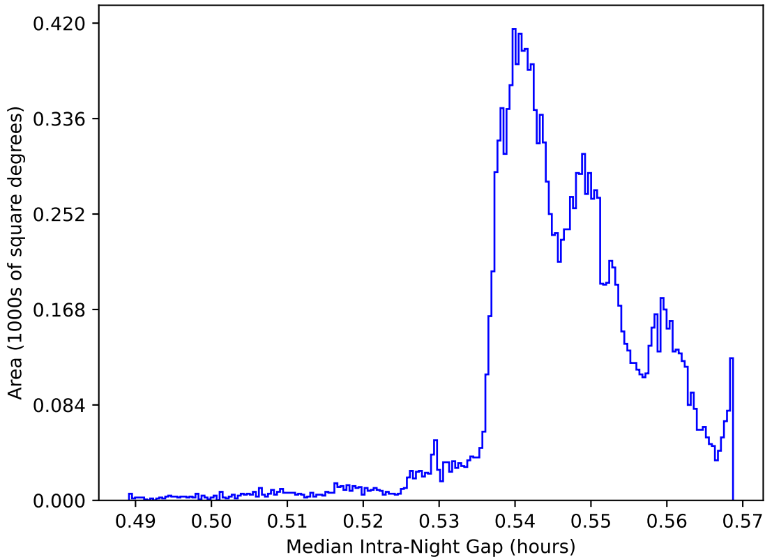
ddf_acor_sf15_ls40_lsr20_v3.4_10yrs WFD: Median Intra-Night Gap
