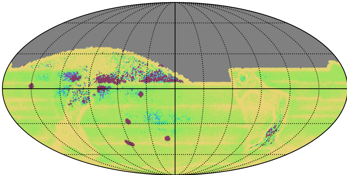
ddf_acor_sf15_lsf40_lsr20_v3.4_10yrs All sky: Median Intra-Night Gap
