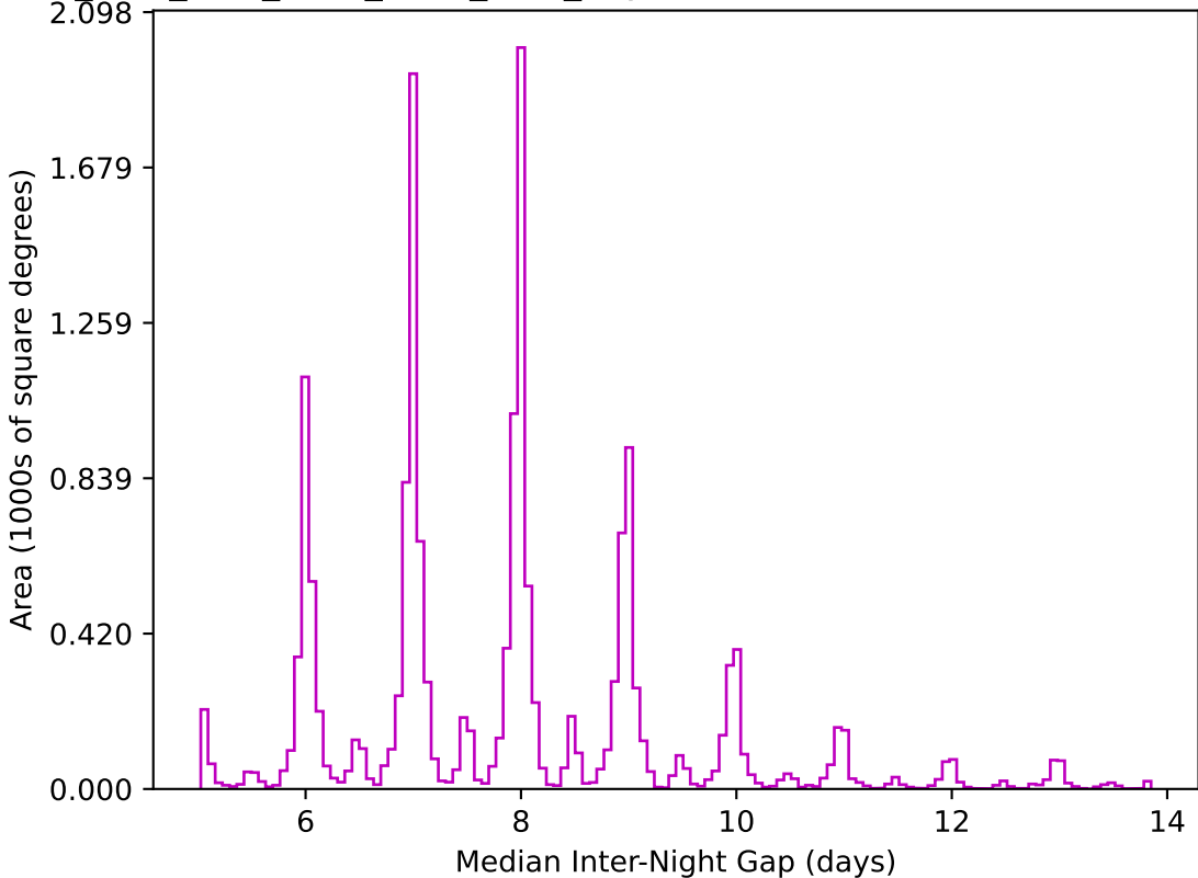
ddf_acor_sf15_lsf40_lsr20_v3.4_10yrs WFD z band: Median Inter-Night Gap
