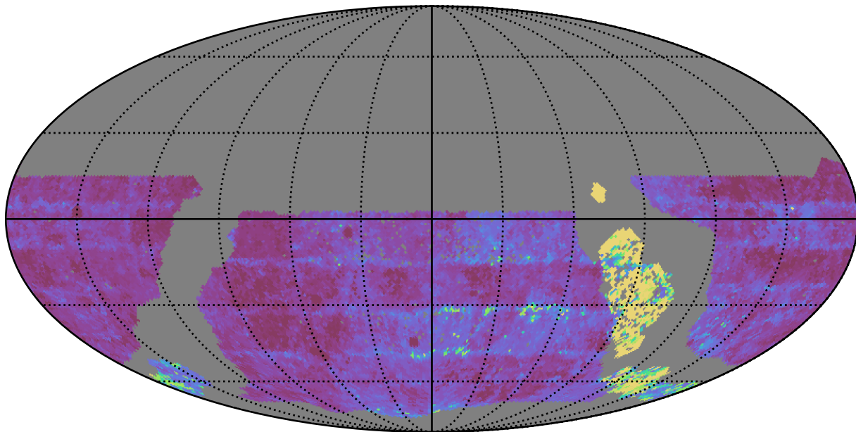
ddf_acor_sf15_lsf40_lsr20_v3.4_10yrs WFD u band: Median Inter-Night Gap
