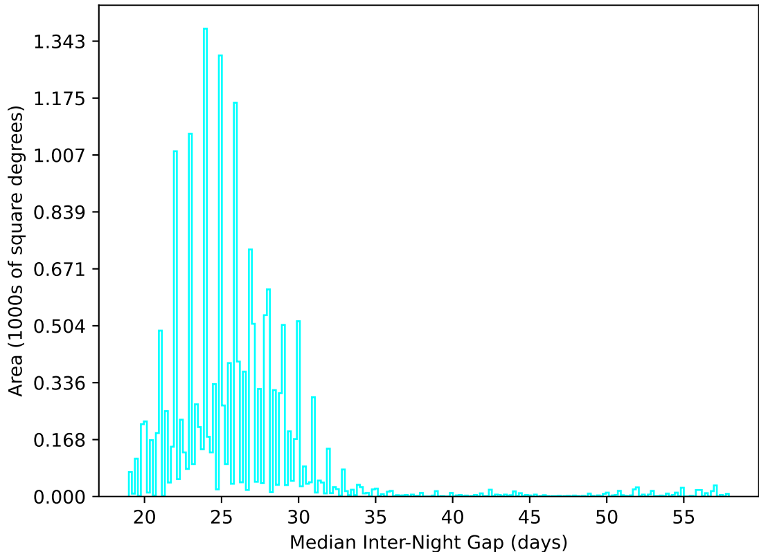
ddf_acor_sf15_lsf40_lsr20_v3.4_10yrs WFD u band: Median Inter-Night Gap
