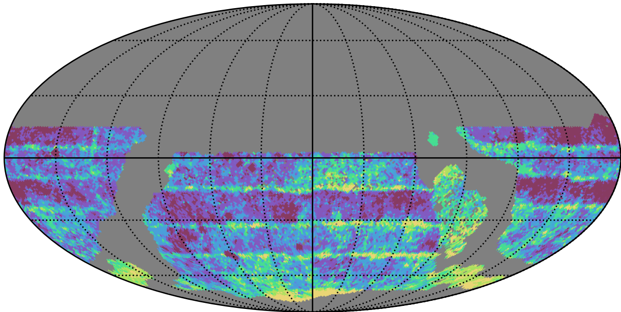
ddf_acor_sf15_lsf40_lsr20_v3.4_10yrs WFD r band: Median Inter-Night Gap
