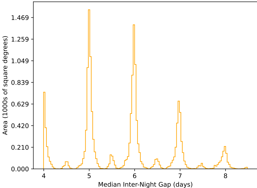
ddf_acor_sf15_lsf40_lsr20_v3.4_10yrs WFD r band: Median Inter-Night Gap
