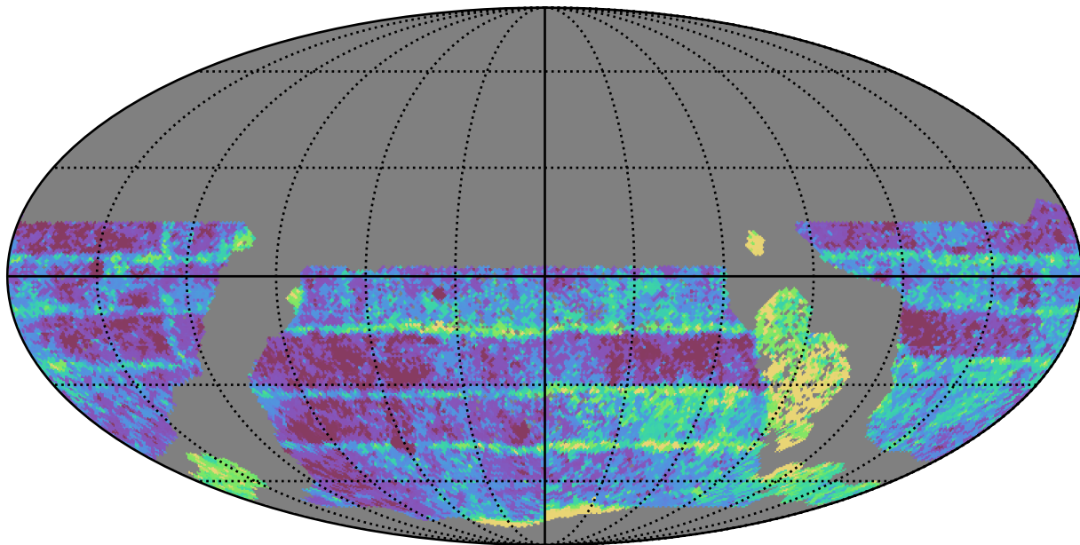
ddf_acor_sf15_lsf40_lsr20_v3.4_10yrs WFD i band: Median Inter-Night Gap
