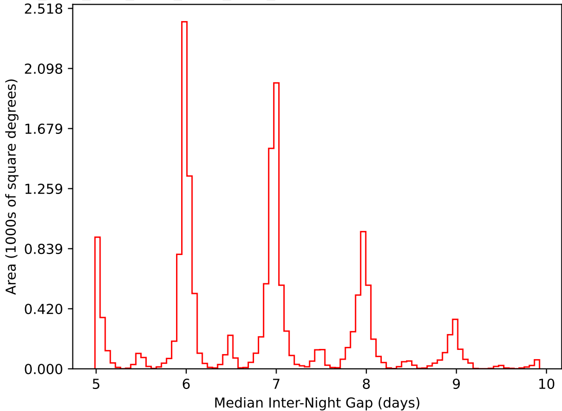
ddf_acor_sf15_lsf40_lsr20_v3.4_10yrs WFD i band: Median Inter-Night Gap
