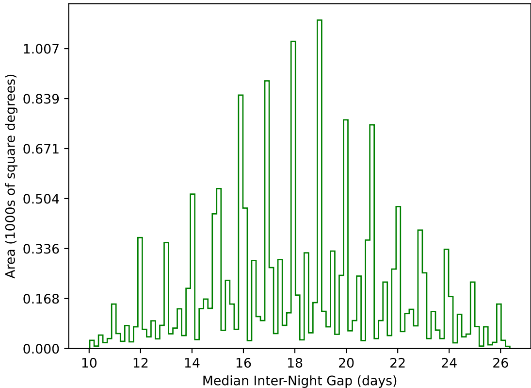
ddf_acor_sf15_lsf40_lsr20_v3.4_10yrs WFD g band: Median Inter-Night Gap
