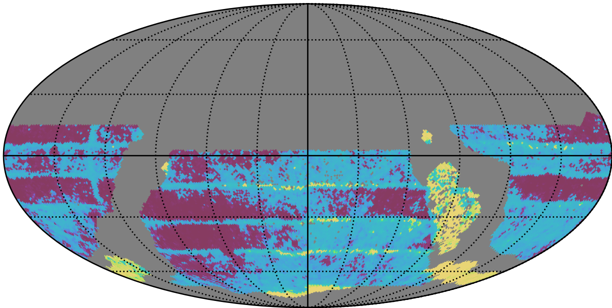
ddf_acor_sf15_lsf40_lsr20_v3.4_10yrs WFD all bands: Median Inter-Night Gap
