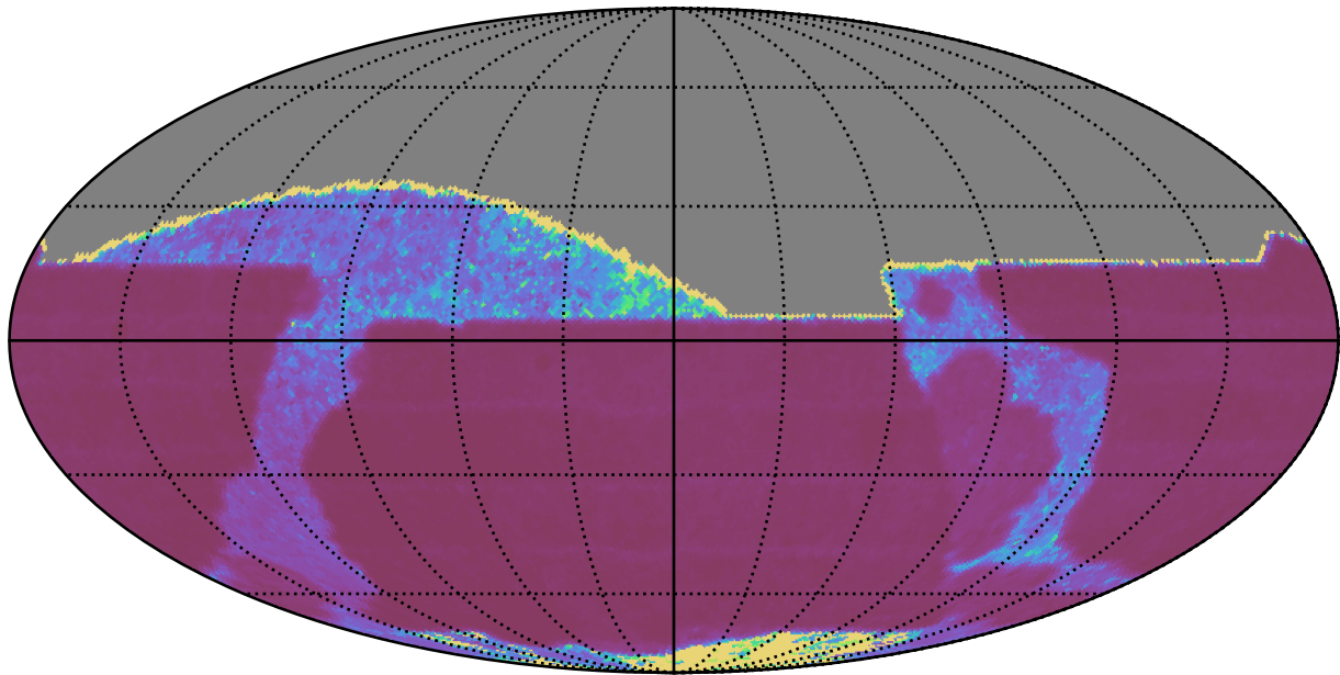
ddf_acor_sf15_lsf40_lsr20_v3.4_10yrs All sky z band: Median Inter-Night Gap
