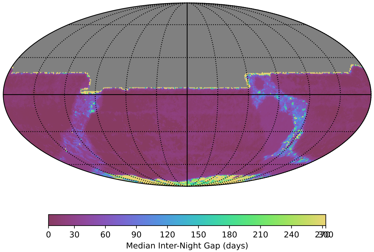
ddf_acor_sf15_lsf40_lsr20_v3.4_10yrs All sky y band: Median Inter-Night Gap
