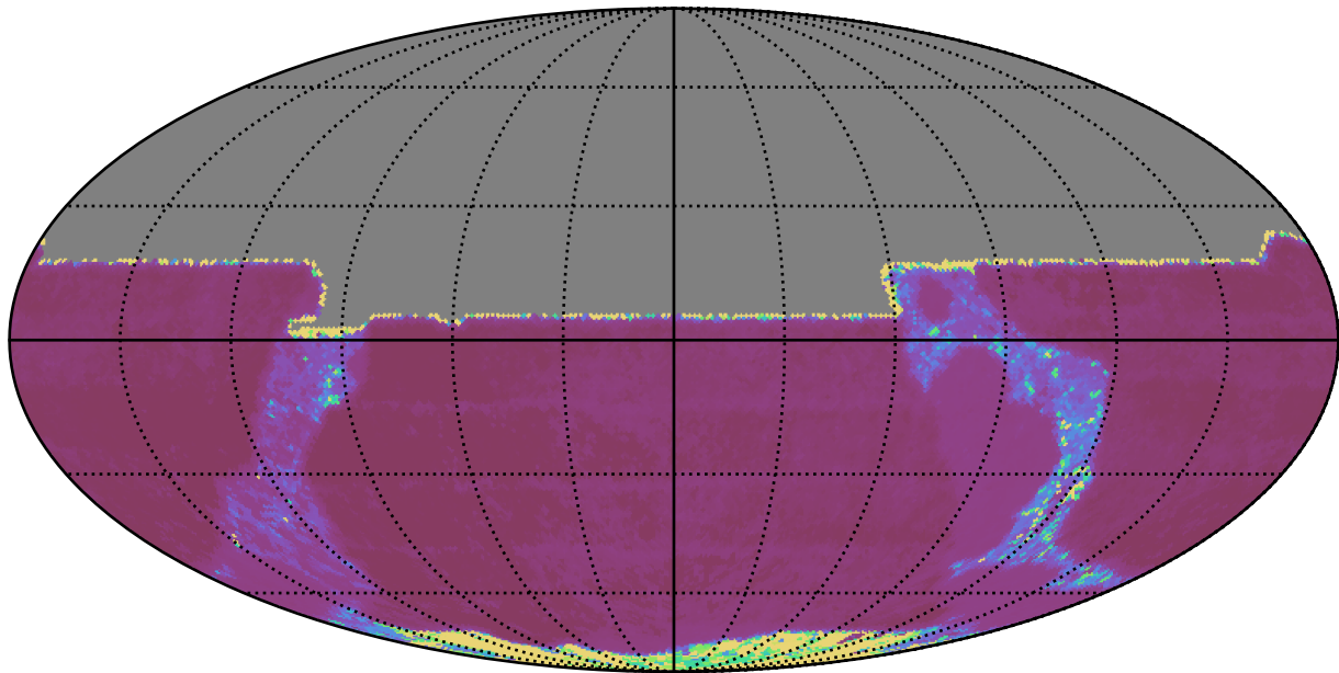
ddf_acor_sf15_lsf40_lsr20_v3.4_10yrs All sky y band: Median Inter-Night Gap
