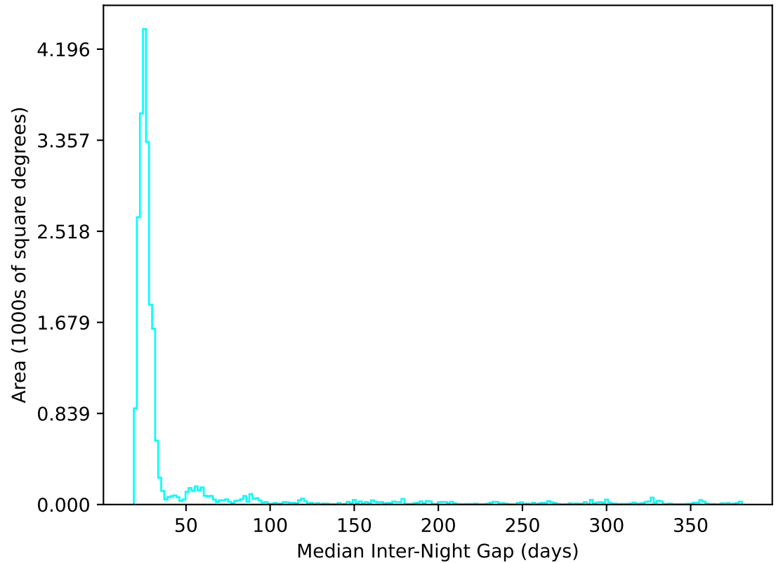
ddf_acor_sf15_lsf40_lsr20_v3.4_10yrs All sky u band: Median Inter-Night Gap
