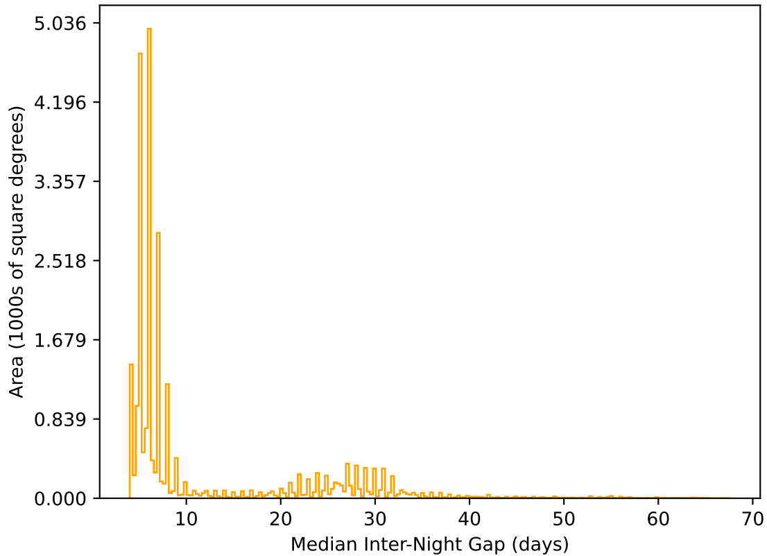
ddf_acor_sf15_lsf40_lsr20_v3.4_10yrs All sky r band: Median Inter-Night Gap
