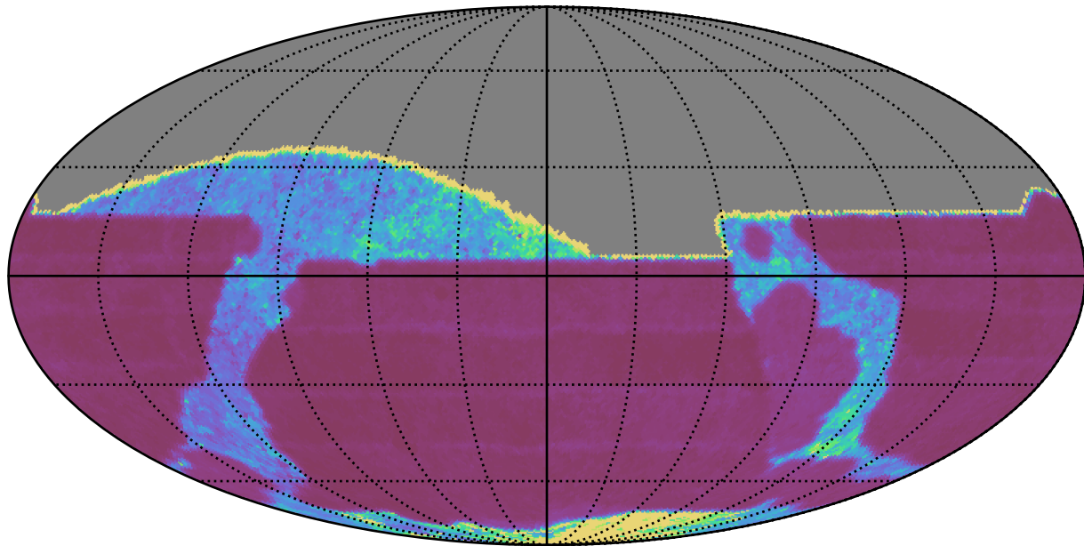
ddf_acor_sf15_lsf40_lsr20_v3.4_10yrs All sky i band: Median Inter-Night Gap
