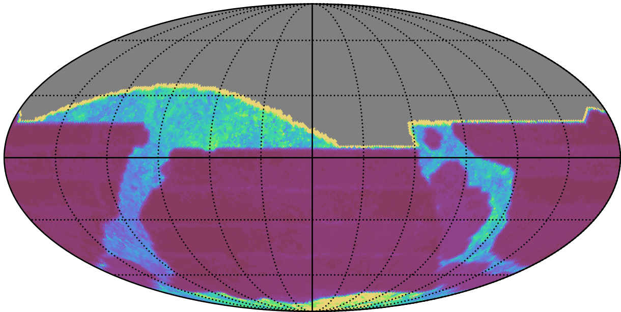
ddf_acor_sf15_lsf40_lsr20_v3.4_10yrs All sky all bands: Median Inter-Night Gap
