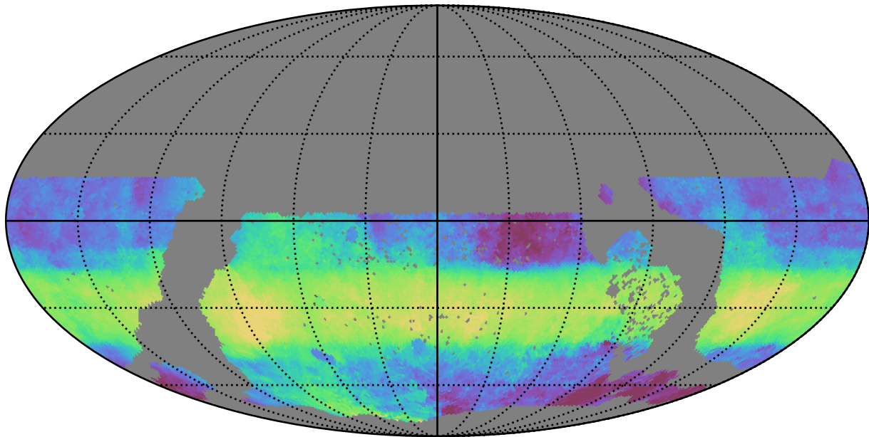
ddf_acor_sf15_lsf40_lsr20_v3.4_10yrs WFD z band: Median HA
