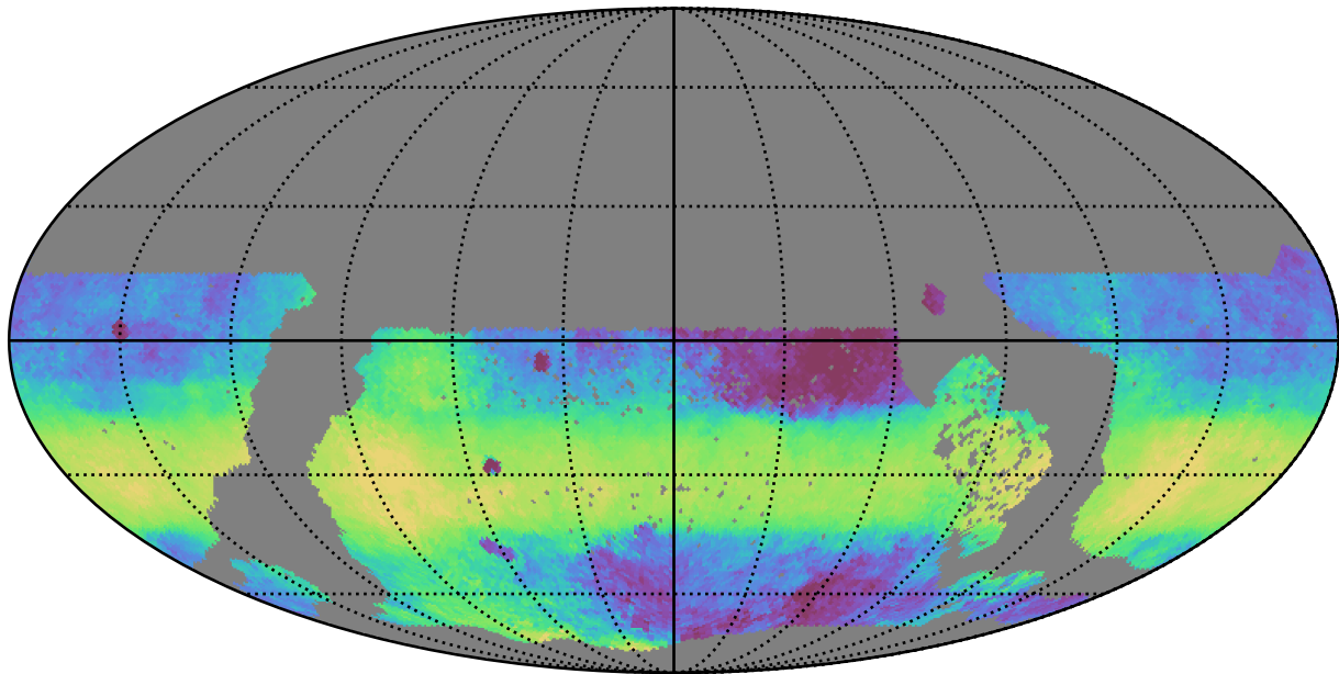
ddf_acor_sf15_lsf40_lsr20_v3.4_10yrs WFD y band: Median HA
