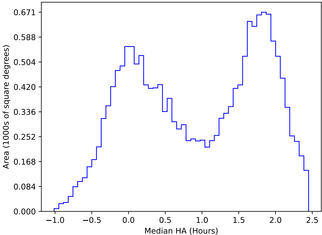
ddf_acor_sf15_lsf40_lsr20_v3.4_10yrs WFD u band: Median HA
