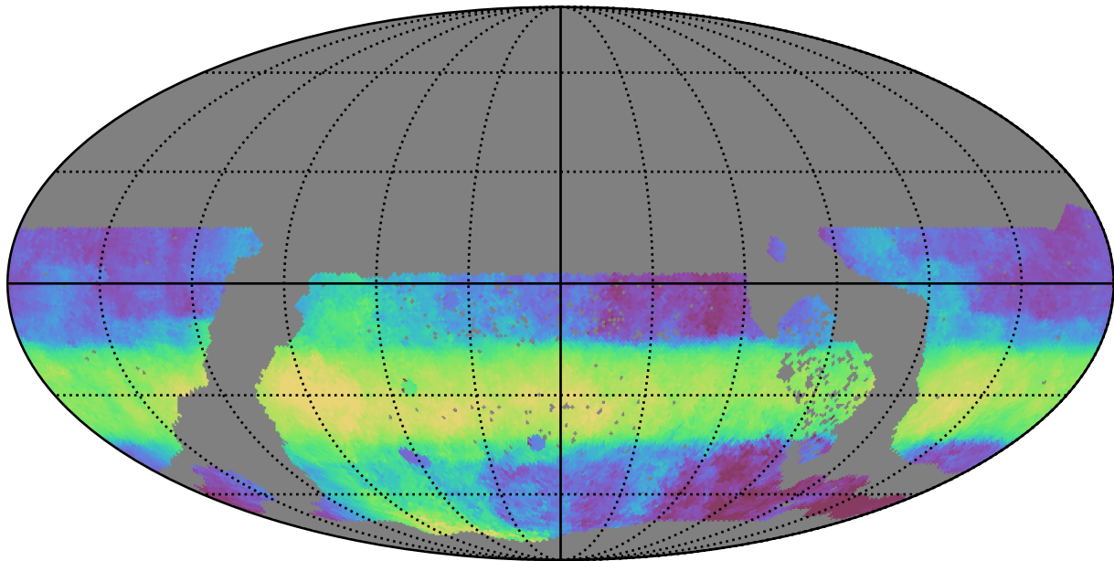
ddf_acor_sf15_lsf40_lsr20_v3.4_10yrs WFD r band: Median HA
