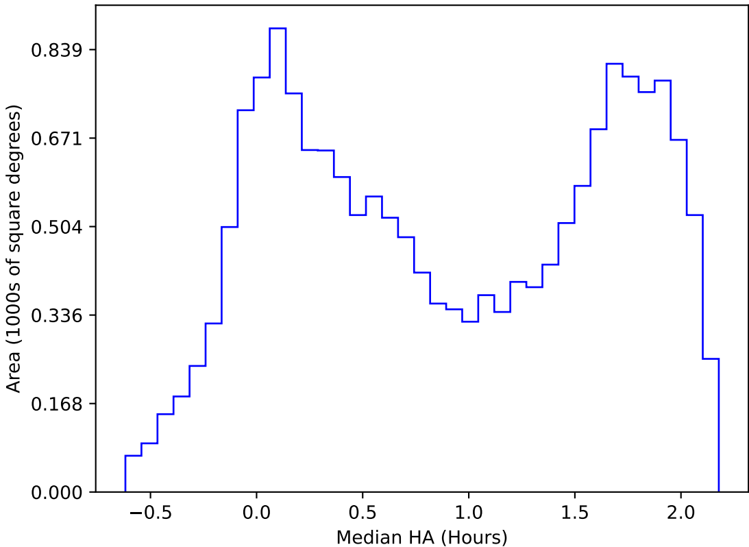
ddf_acor_sf15_lsf40_lsr20_v3.4_10yrs WFD r band: Median HA
