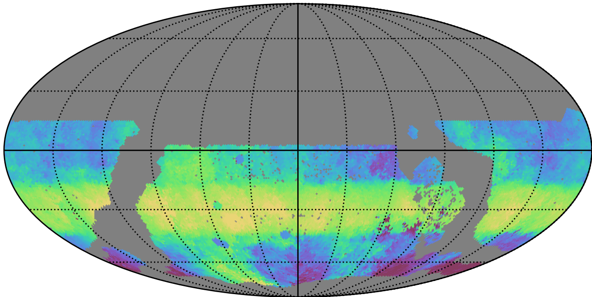
ddf_acor_sf15_lsf40_lsr20_v3.4_10yrs WFD g band: Median HA
