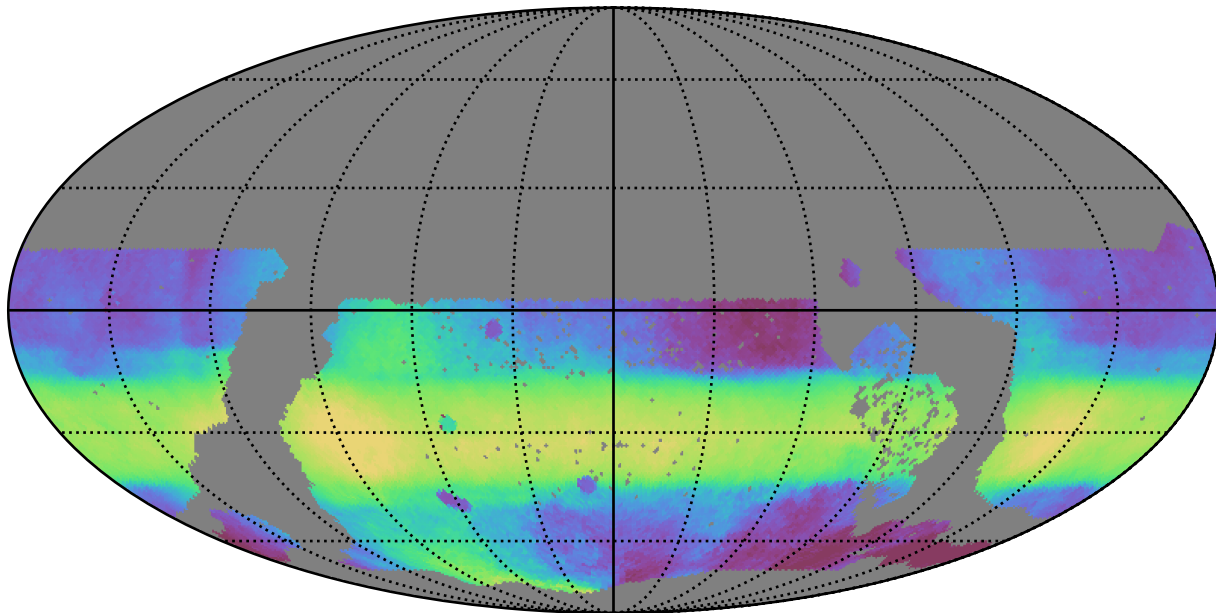
ddf_acor_sf15_lsf40_lsr20_v3.4_10yrs WFD all bands: Median HA
