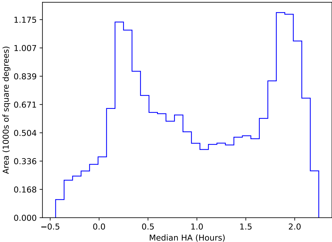
ddf_acor_sf15_lsf40_lsr20_v3.4_10yrs WFD all bands: Median HA
