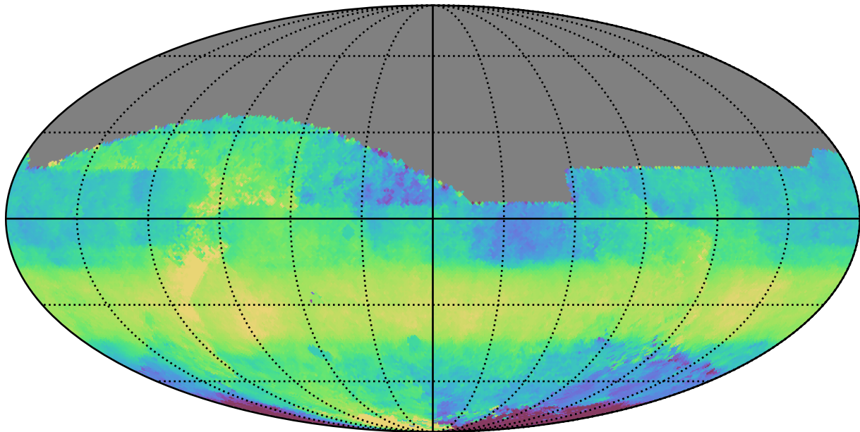
ddf_acor_sf15_lsf40_lsr20_v3.4_10yrs All sky z band: Median HA
